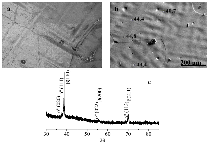
Fig. 1. The image of microstructure (a), concentration of Nb (mas %) in the elements of structure (b) and fragment of X-ray diffraction pattern (c) of the cast specimen
